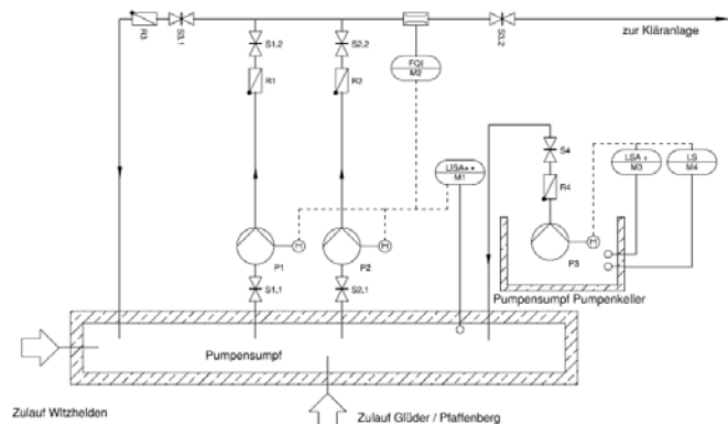
R+I-Schema
